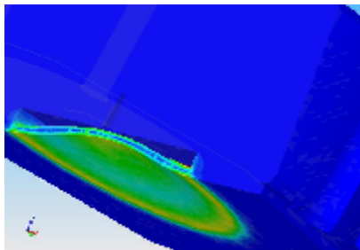
Picture 4: Metallux FEM simulation of optimising base plate geometry
