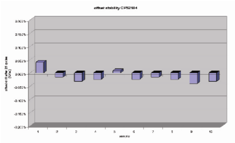
Picture 2: Metallux AG Offsetstability after temperature change at 85% relative moisture
