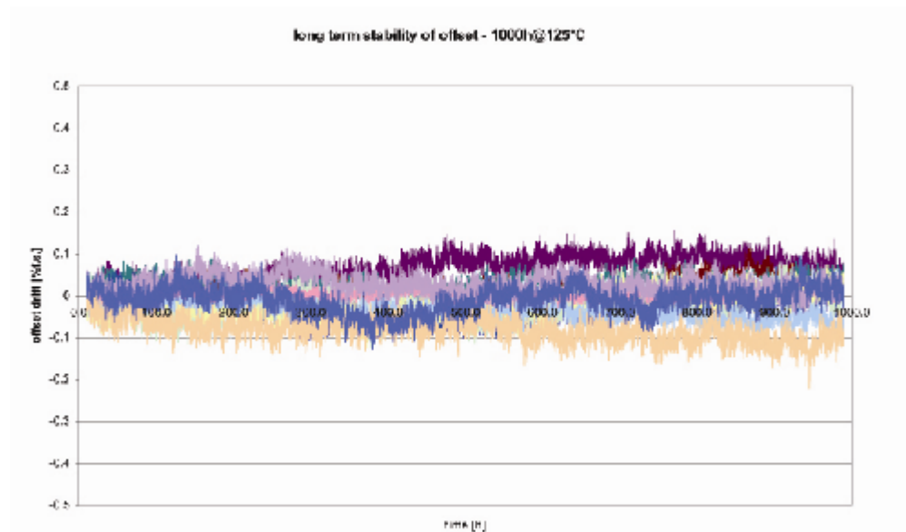
Picture 5: Long term stability of the offset-signal of monolithic and flush mounted ceramic pressure sensors manufactured by Metallux AG
