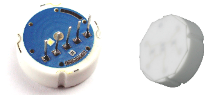
Picture 3: Metallux CPS2184 with flush mounted membrane (front-and rear view)
